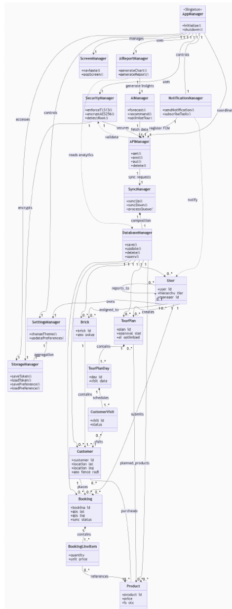
Figure 5.2: Comprehensive Class Diagram of the Konvert Ecosystem
